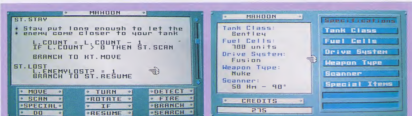
Above: In the design module. Here you attempt to give your tank some artificial intelligence that it will use once it's on the battlefield. This is part of a scanning routine that tells your tank to wait for the enemy to come to it - a good plan for getting the first few shots in on the enemy. This screen is also where you juggle your credits and get the best weapons your clearance level allows.
